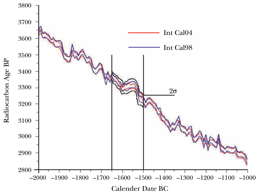
Fig. 3 Comparison of INTCAL98 and INTCAL04 calibration curves, with the addition of a two sigma range in the span between 1500 and 1650 (after S. MANNING in: The Thera (Santorini) Volcanic Eruption and the Absolute Chronology of the Aegean Bronze Age , a companion website to MANNING 1999, http://www.arts.cornell.edu/classics/Faculty/SManning_files/testoftime.pdf )
