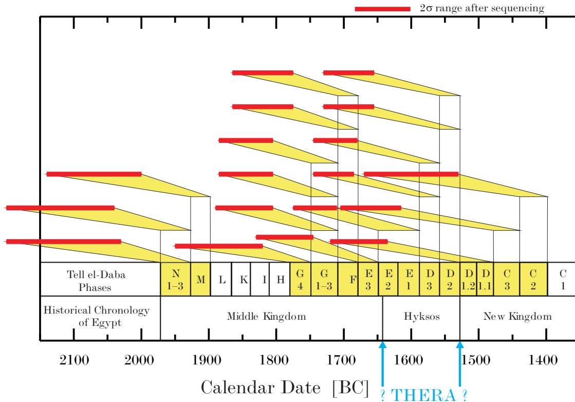
Fig. 2 Comparison of calibrated two sigma 14 C ranges with the historical chronology of Egypt and the corresponding Tell el-Dab a phases
