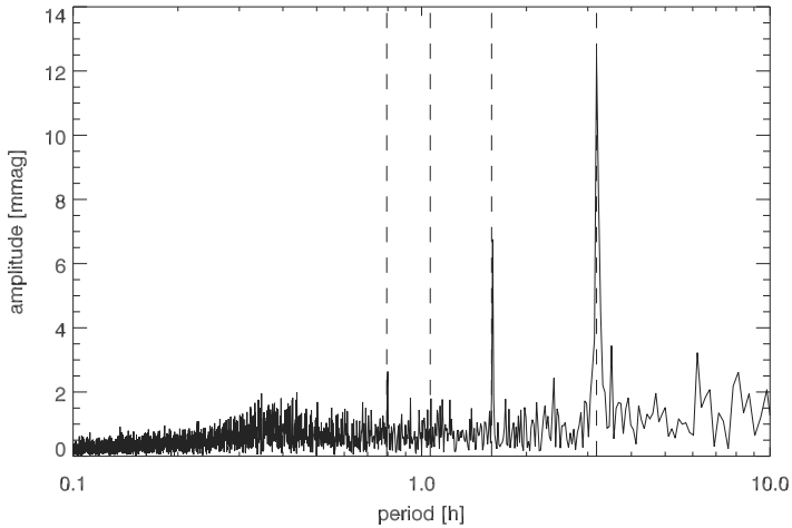
Figure 1: Periodogram derived from the DFT analysis. The main period and its harmonics are indicated by dashed lines.
