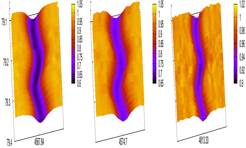
Figure 1: Examples of line-profile variations affecting Si III \lambda 4567.8, 4574.7 and 4813.3 on 5 October 2007.
