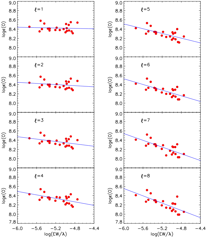
Figure 6: Estimation of the microturbulent velocity from the O II lines.
