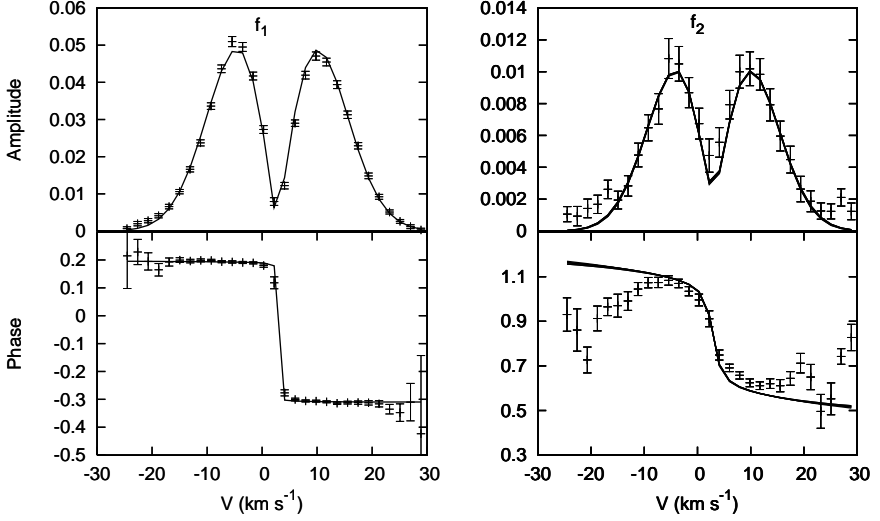
Figure 2: Amplitude and phase distributions (points with error bars) across the C II \lambda 5145 Å line, for the frequencies f_1 = 6.58974 and f_2 = 0.68241 d ^{-1} . The bestfit model is represented by full lines. For f_1 , the mode is radial. For f_2 , the differences between the best solutions listed in Table 2 for (\ell_2, m_2) = (1, 1) , (2, -1) and (2, -2) are smaller than the thickness of the lines. The amplitudes are expressed in units of continuum and the phases in \pi radians.
