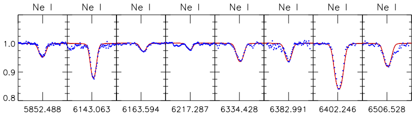
Figure 9e: Same as Fig. 9a, but for the Ne I lines.
