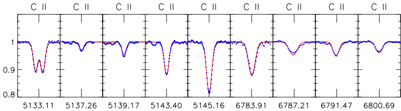
Figure 9b: Same as Fig. 9a, but for the C II lines.
