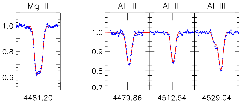
Figure 9f: Same as Fig. 9a, but for the Mg II (left) and Al III (right) lines.
